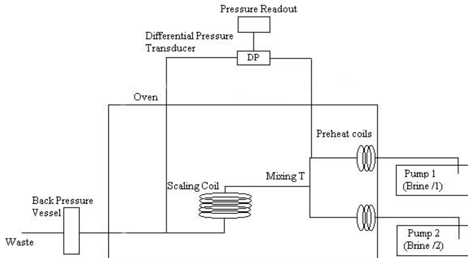
A Simple Schematic of the Dynamic Tube Blocking Rig
